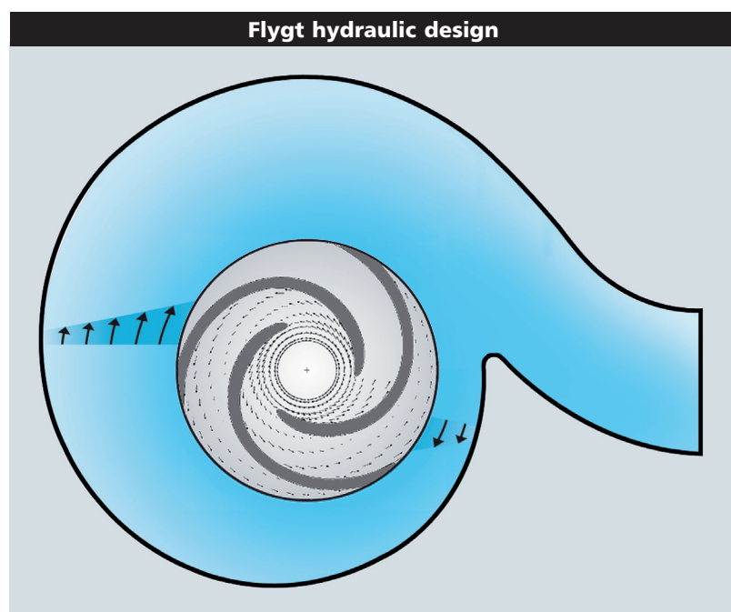
Swept-back impeller design and larger volute mean more homogeneous flow with less wear to all contact surfaces.
